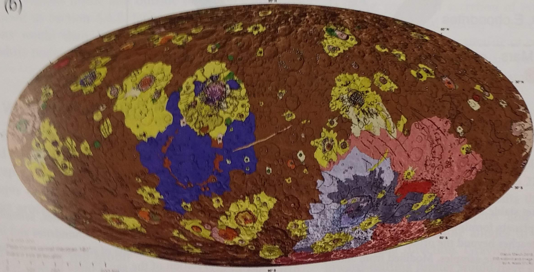
GEOLOGIC MAP of CERES Global dataset based on quadrangle mapping -
