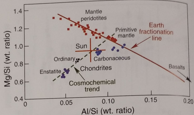
Figure 5.9 Mg/Si versus Al/Si for chondrites and terrestrial mantle rocks. Intersection of the cosmochemical and fractionation trends serves as an estimate of the primitive mantle composition. Modified from Righter et al. (2006).
