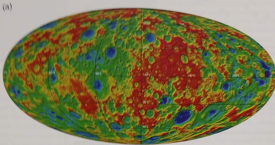
-7.5 km 7.5 km Elevation [km]
