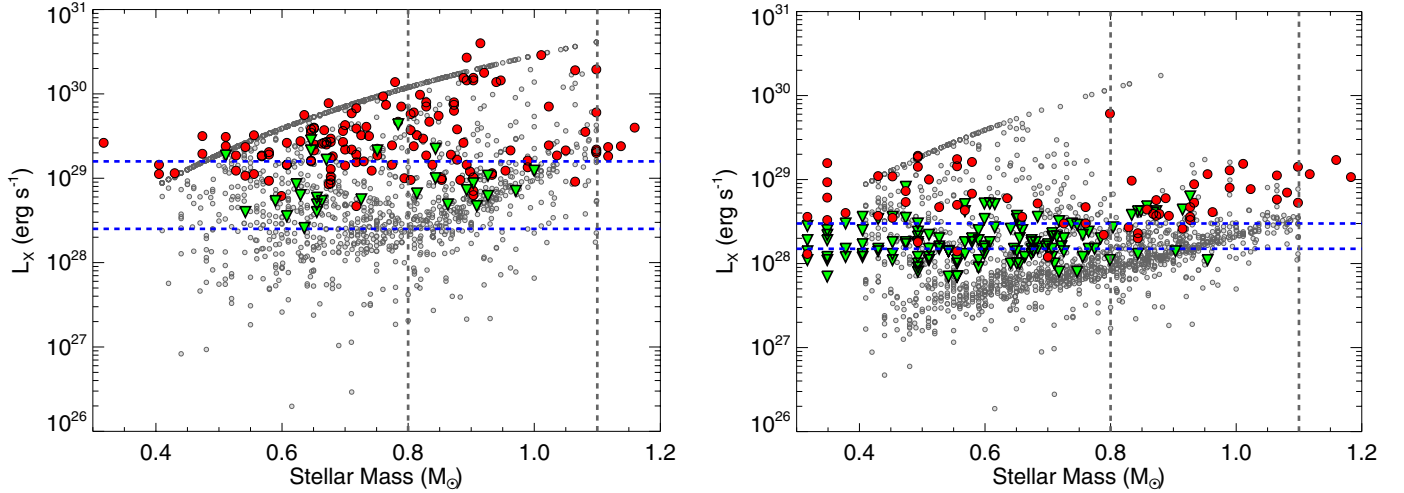
Fig. 1. Comparisons between observed and predicted distributions of L_X at ages of 150 Myr ( left ) and 620 Myr ( right ). The grey symbols show predicted distributions calculated using Eq. (1) and the distributions of rotation rates derived by Johnstone et al. (2015). The red circles and green triangles show detections and upper limits for stars in the Pleiades ( left ) and Hyades ( right ). The horizontal blue lines show detection thresholds. The upper line of stars in the theoretical distributions is caused by the stars whose rotation rates lie above the mass dependent saturation threshold.
