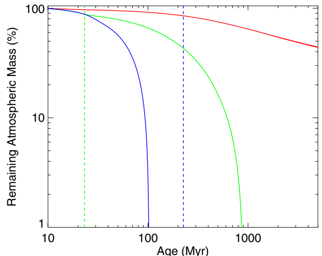
Fig. 4. Evolution of the planetary atmospheric mass of a 0.5 M_{\text{Earth}} planet orbiting a 1 M_{\odot} star at 1 AU with an initial mass of 5 \times 10^{-3} M_{\text{Earth}} . The tracks correspond to planets orbiting stars that are in the 10th (red), 50th (green), and 90th (blue) percentiles of the rotational distributions. The vertical lines show the stellar saturation times.
