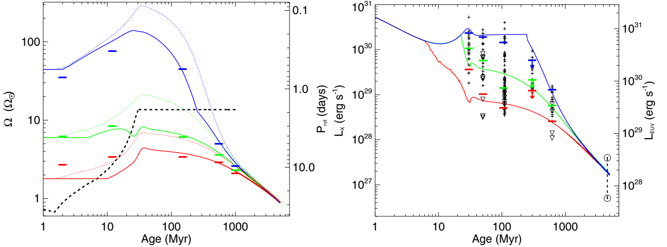
Fig. 2. Left: predicted rotational evolution tracks for stars at the 10th (red), 50th (green), and 90th (blue) percentiles of the rotational distribution. The solid and dotted lines show the envelope and core rotational evolution, respectively, and the horizontal solid lines show the observational constraints on the percentiles. The dashed black line shows the time dependent saturation threshold for \dot{M} , B_{\text{dip}} , and L_X calculated assuming a constant saturation Ro and the \tau_* values of Spada et al. (2013). Right: predicted L_X along each of our rotation tracks and comparisons to observed L_X values of single stars in several clusters with upper limits shown by \nabla symbols. The solid horizontal lines show the 10th, 50th, and 90th percentiles of the observed distributions of L_X at each age calculated by counting upper limits as detections. The two solar symbols at 4.5 Gyr show the range of L_X for the Sun over the course of the solar cycle. The scale on the right y -axis shows the associated L_{\text{EUV}} .
